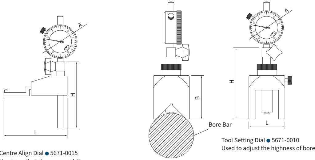
Centre Align Dial ● 5671-0015 Used to adjust the concentricity of cylinder bore and bore bar
